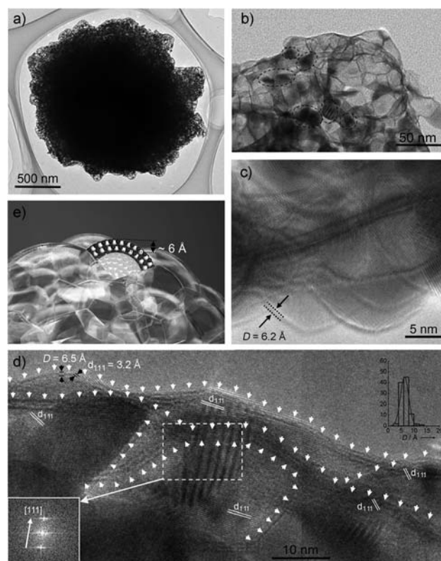
Figure 2. a,b) Typical TEM images with different magnification. c,d) Typical high-resolution TEM images. e) Digital camera photograph of soap bubble with a model of the wall of \text{CeO}_2 foam inserted. Insets in (d): FFT patterns obtained from the HRTEM image and statistical analysis of thickness distribution of walls of \text{CeO}_2 foam (average D = 6.41 \text{ \AA} , relative standard deviation (22.5%) derived from counting 50 walls and two different points of each wall were measured. The areas marked by black dotted circles in (b) indicate some small particles in the \text{CeO}_2 foam. The vertical stripes located in the dotted frame in (d) indicate the Moiré patterns frequently observed in TEM images.
